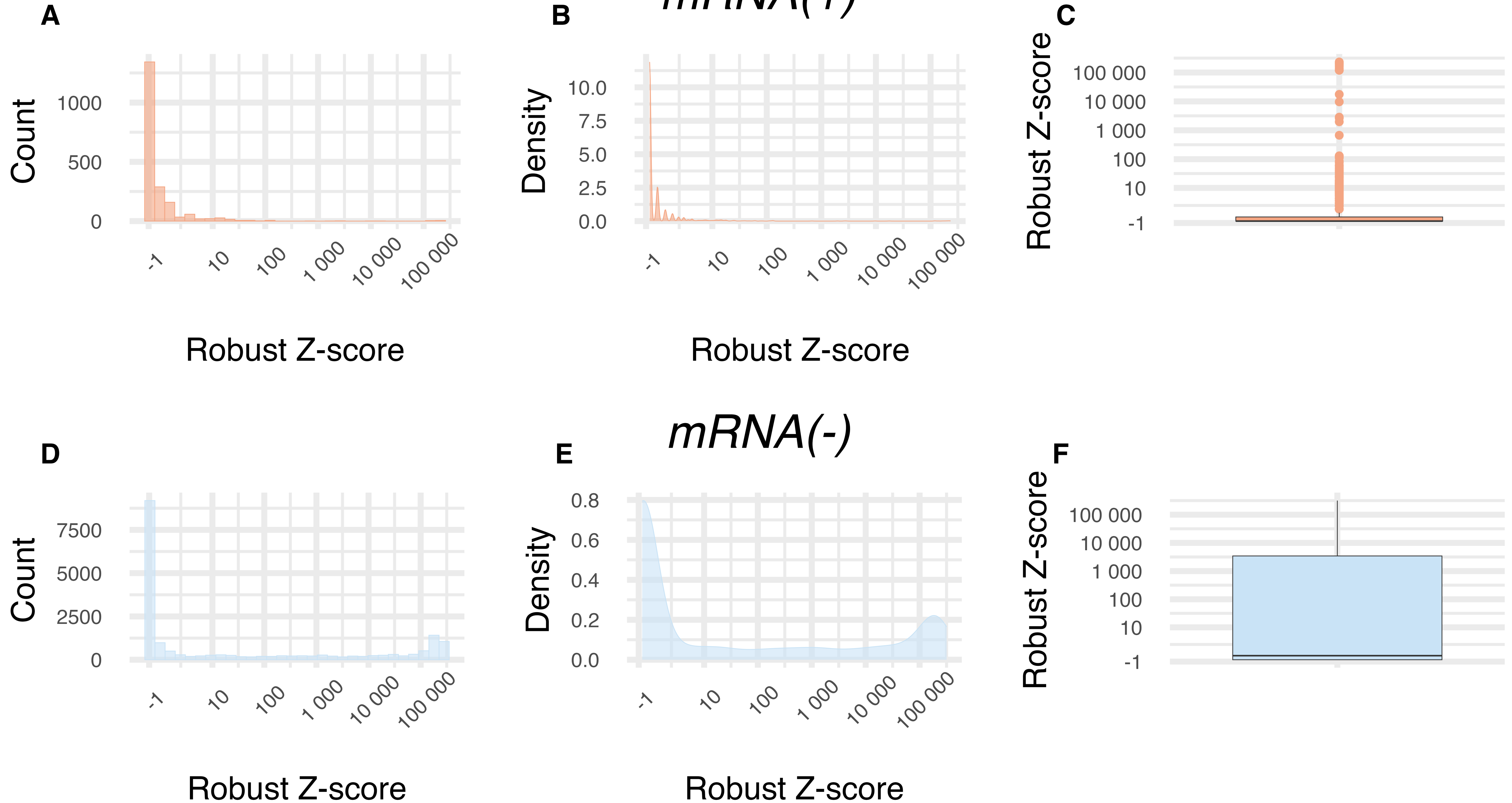
Supplementary Figure S9. mRNA copies robust z-scores distributions in log scale. A-C) Histogram, Density and Boxplot for mRNA(+), D-F) Histogram, Density and Boxplot for mRNA(-). The positive dataset shows log (robust z-scores) centered around 0.1 which also applies for the negative set. It is important however to highlight that there is greater spread for negative set compared to the positive set, which indicates the two dataset come from different distributions.
